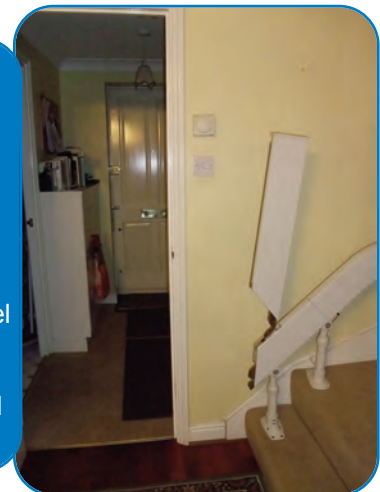
Our curved tracked stairlifts will fit most staircases, with a motorized hinge being an ideal solution when the track covers a doorway. All our stairlifts swivel at the top of the stairs, this provides safe transfer on and off the stairlift.
